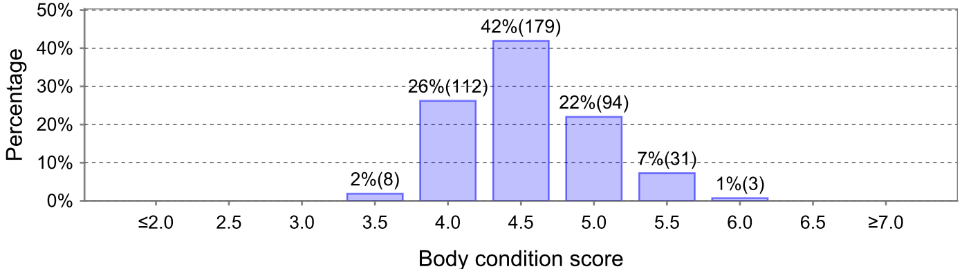
27 Nov 17 (427 animals - identified, average: 4.5)
