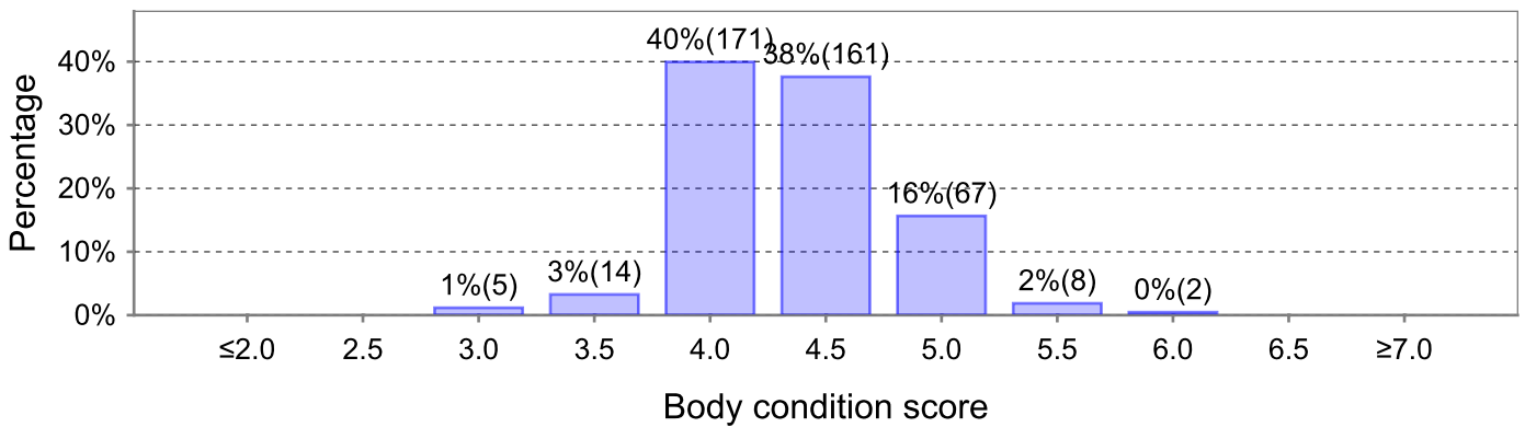
26 Mar 18 (425 animals - identified, average: 4.3)
