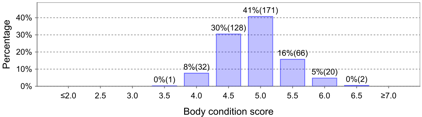
25 Sep 17 (385 animals - identified, average: 4.6)
