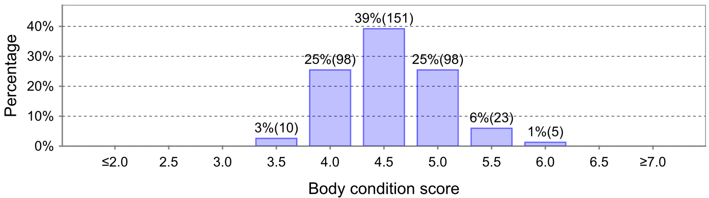
30 Oct 17 (429 animals - identified, average: 4.4)
