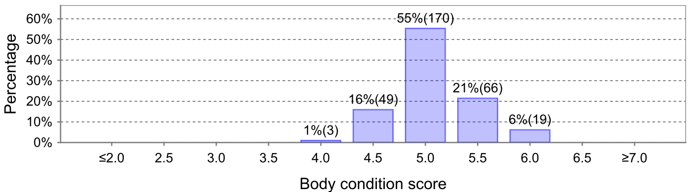
20 Jul 17 (307 animals - identified, average: 5.1)
