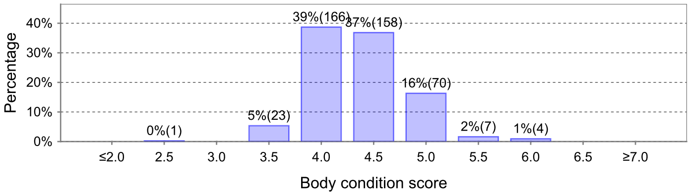
1 Mar 18 (428 animals - identified, average: 4.4)
